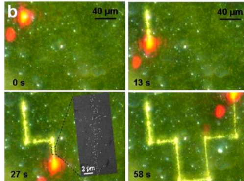
Fig. 3. Real-time patterning of gold nanoparticles (mixture of 60 nm and 90 nm in diameter) using a manually controlled laser spot. The field gradients formed in the vicinity of the optically defined virtual electrodes interact with the nanoparticles, trapping them in the potential well. The particles are strongly attracted to the surface by the immobilization force consisting of DEP and electrophoresis forces. [14]
