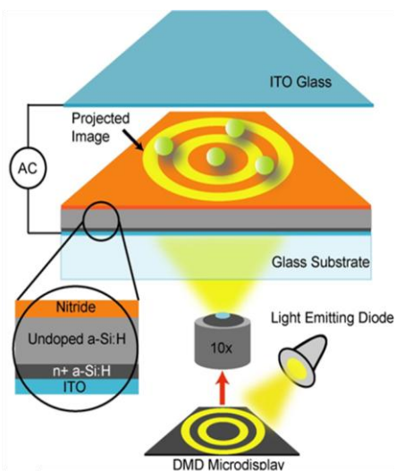
Fig. 1. OET use the selective illumination of a photoconductive layer to create ‘virtual electrodes’ for dielectrophoresis. Parallel manipulation of cells can be realized using projected optical images. [1]
